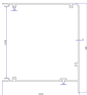
PG004 - INTERIOR GUIDE FOR GUILLOTINE REF:37268
