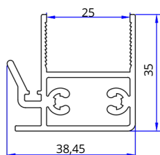
PG010 - GUILLOTINE GUIDE COVER REF:37270
