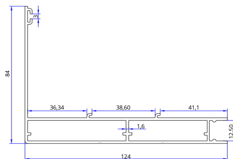
PG006 - GUILLOTINE LOWER FRAME REF:37263
